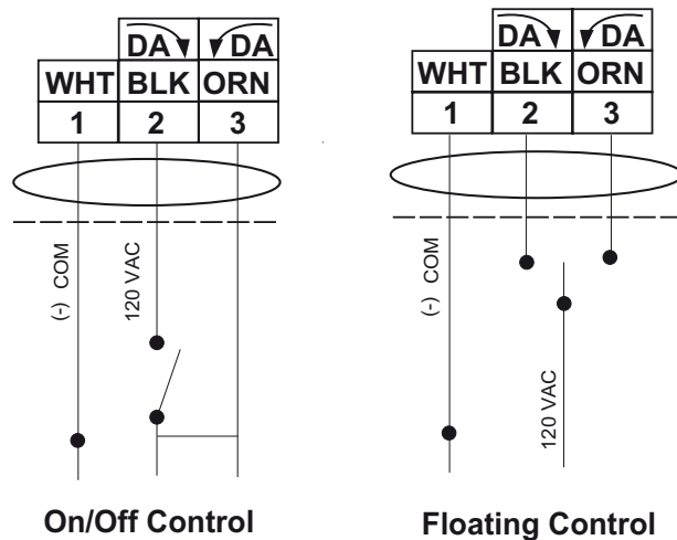
Figure 1: VA93xx-AUA-2x wiring diagrams
