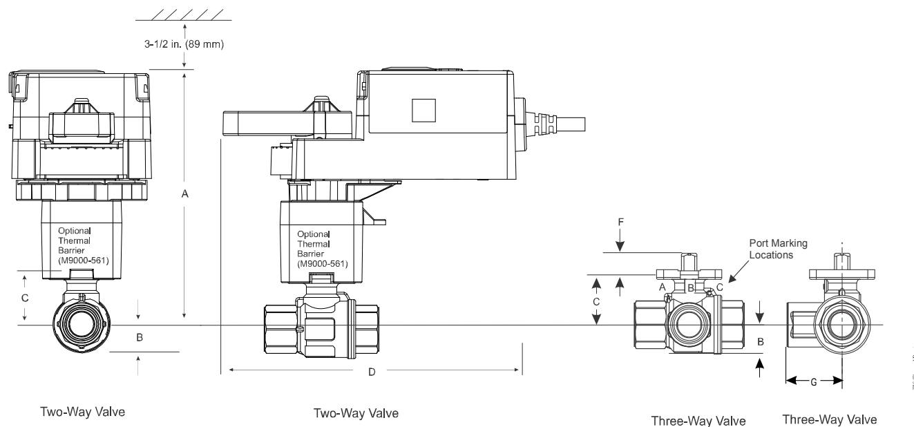
Figure 6: VA9300 Series Electric Non-Spring Return Actuator and Valve Dimensions (with Optional M9000-561 Thermal Barrier)
