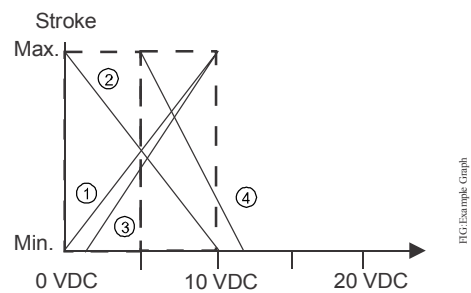
Figure 5: Graphed Examples of Table 3 Command Signals
