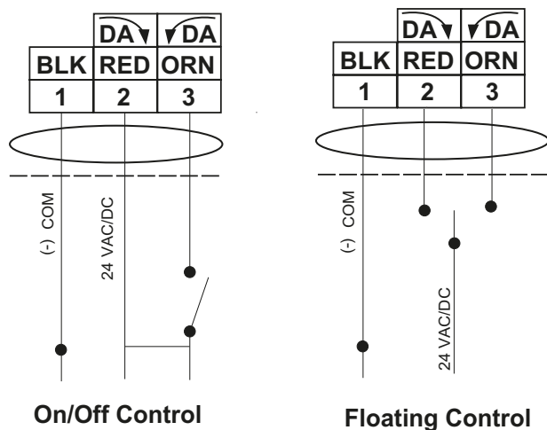
Figure 1: VA93xx-AGA-xx wiring diagrams
