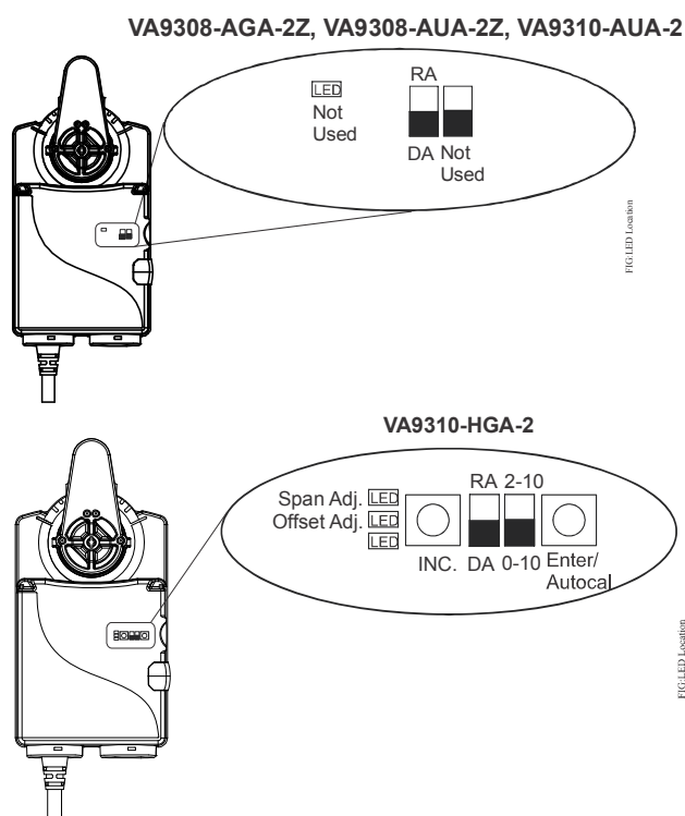
Figure 4: DIP Switches and LEDs
